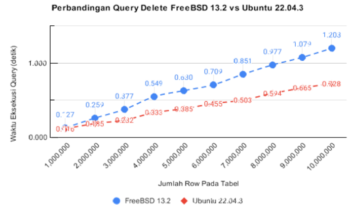
Gambar 6 Perbandingan Query Delete FreeBSD 13.2 vs Ubuntu 22.04.3
