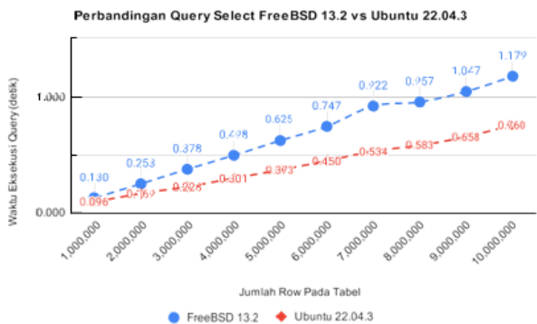
Gambar 4 Perbandingan Query Select FreeBSD 13.2 vs Ubuntu 22.04.3
