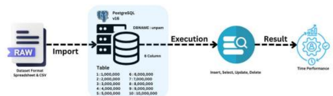
Gambar 1 Detail Pengolahan Data-Tabel-Query
