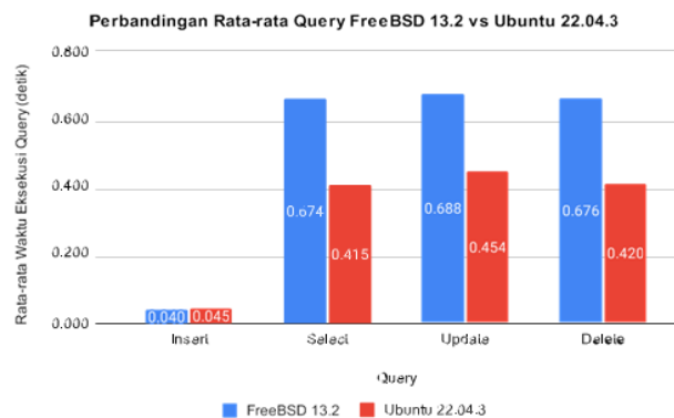
Gambar 7 Rata-rata performa Query Insert, Select, Update, Delete
