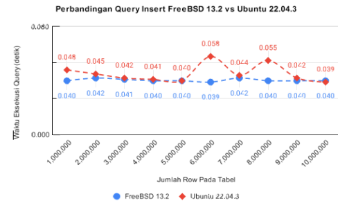
Gambar 3 Perbandingan Query Insert FreeBSD 13.2 vs Ubuntu 22.04.3
